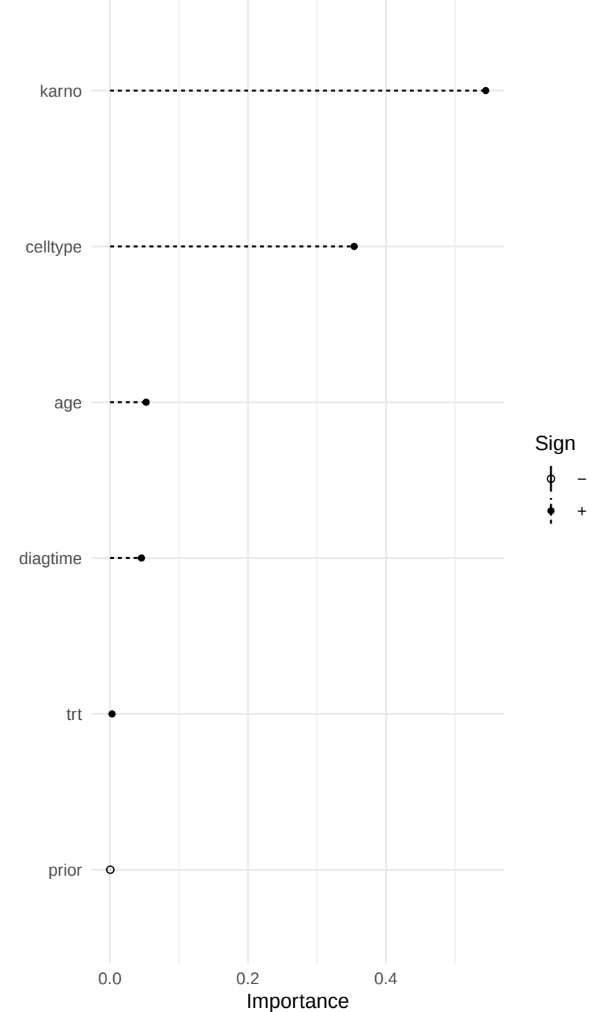
Variable Importance – RandomForestSRC
