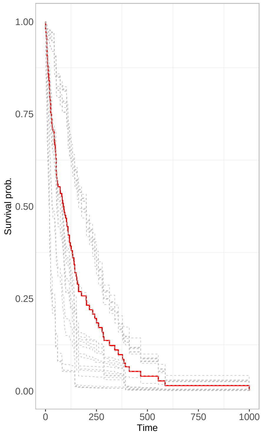
Survival Curves – RandomForestSRC
