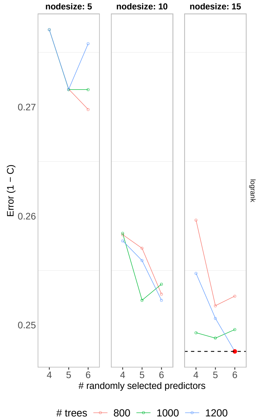
Tuning Results – RandomForestSRC
