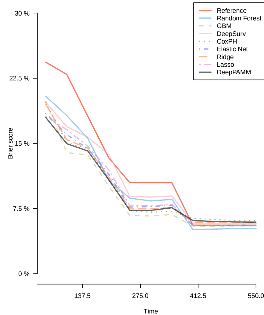
Brier score over time
