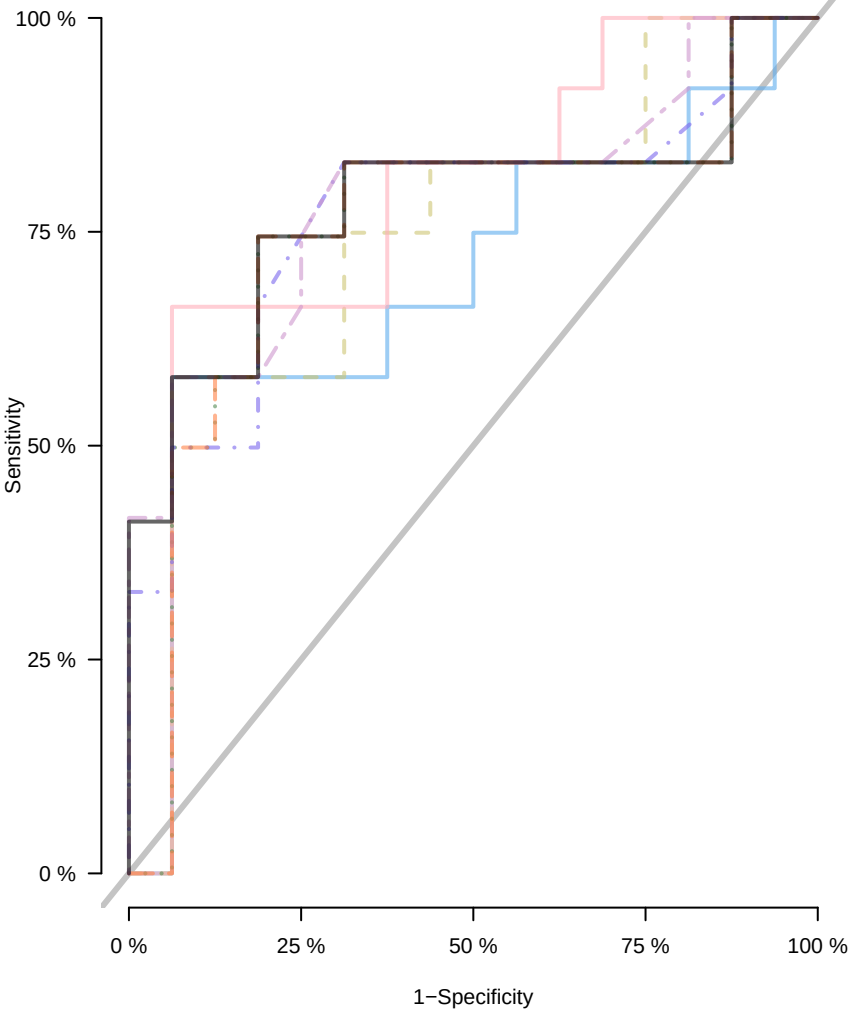
ROC at time = 50
