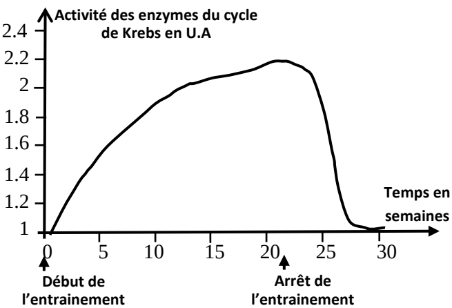
Document 3
