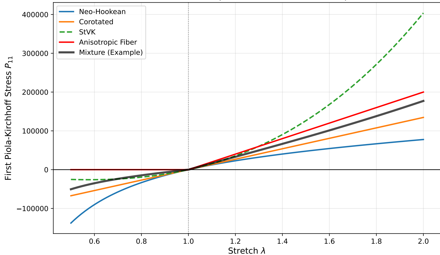
Stress-Stretch Comparison of Constitutive Experts
