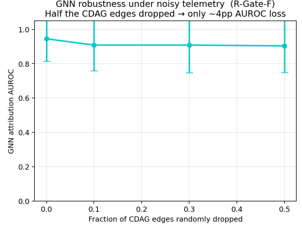
Fig. 7. GNN attribution AUROC vs fraction of CDAG edges randomly dropped (proxy for missing activation telemetry). Half the edges removed costs \sim 4 AUROC points.
