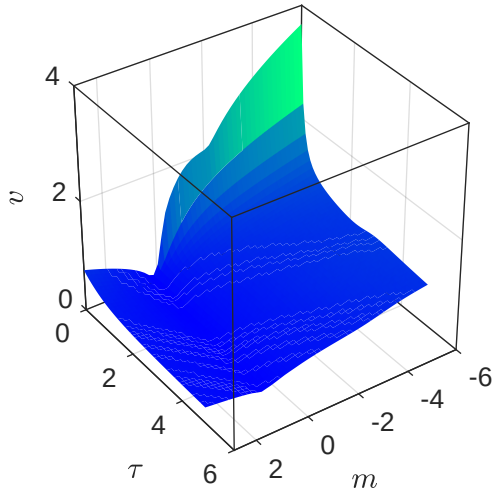
Multi (no regularization)
