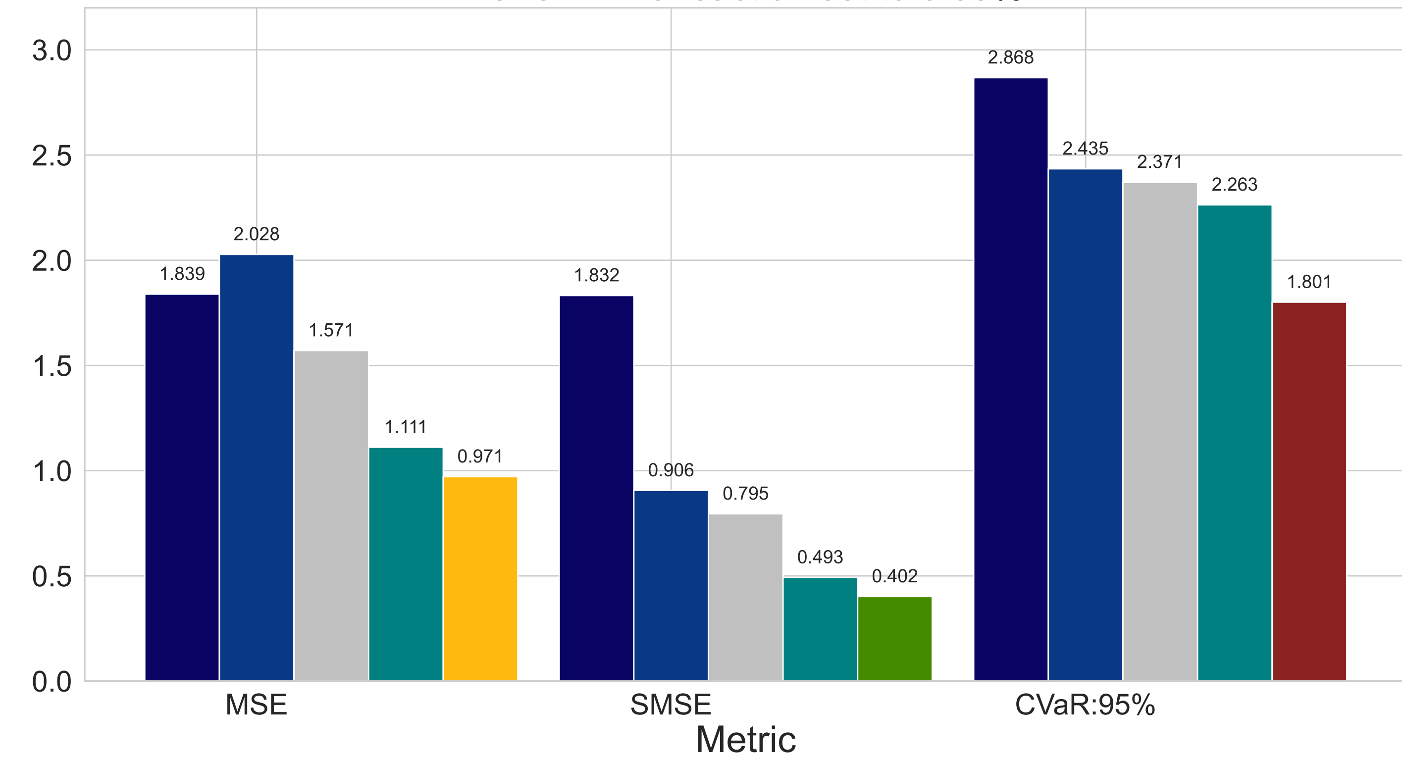
Panel B: Transaction set to 0.05%
