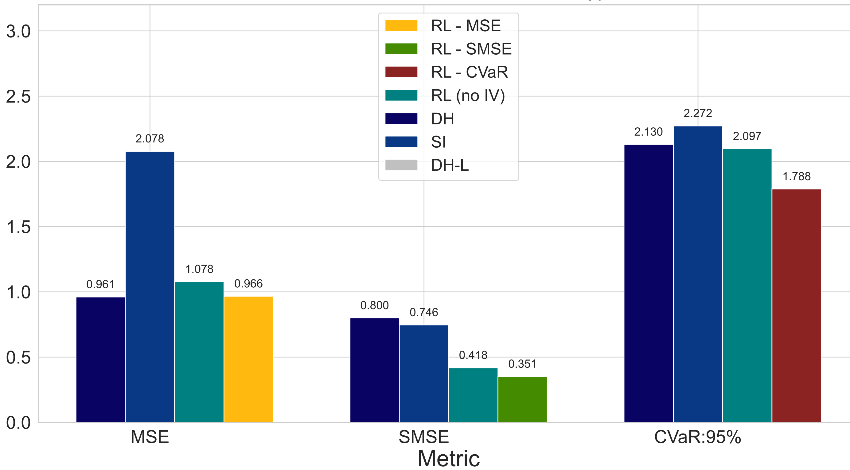
Panel A: Transaction set to 0%
