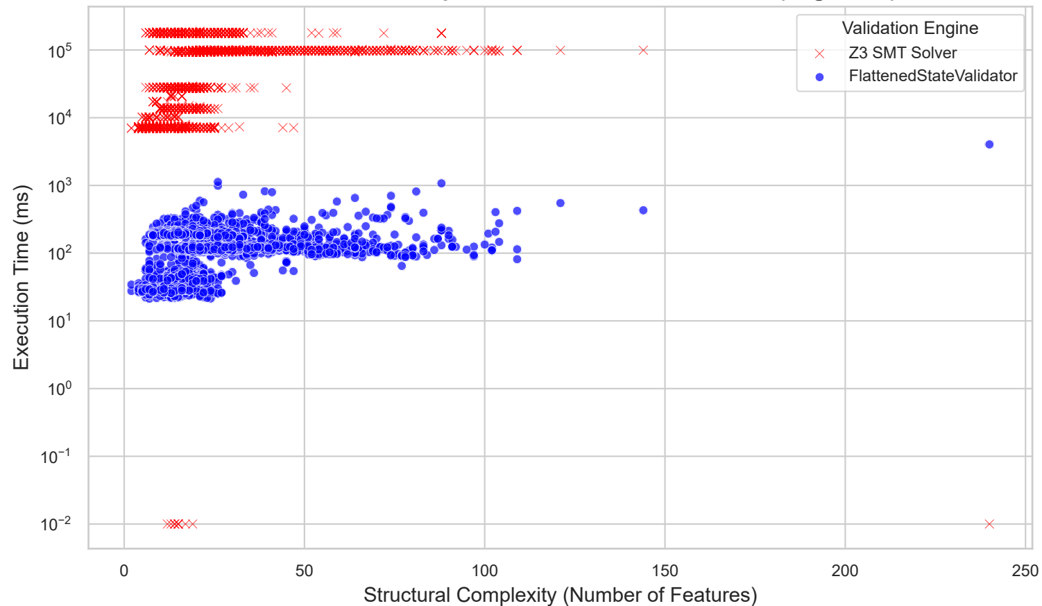
Execution Time Comparison: Z3 vs. Native Validator (Log Scale)
