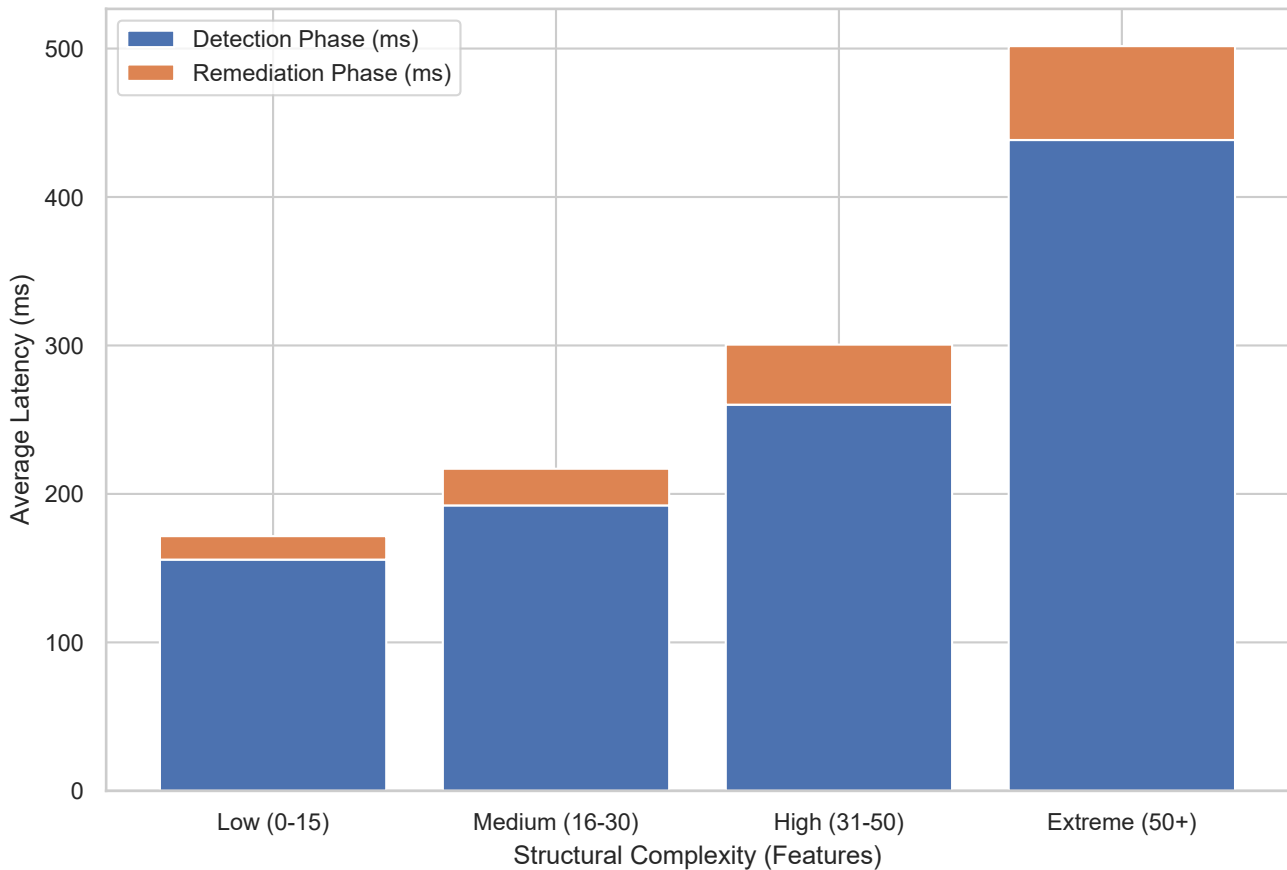
End-to-End Pipeline Latency by Structural Complexity
