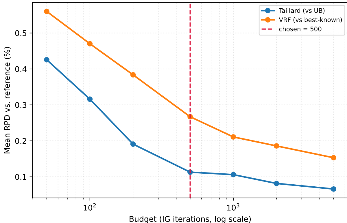
EXP-003: mean RPD vs budget by benchmark
