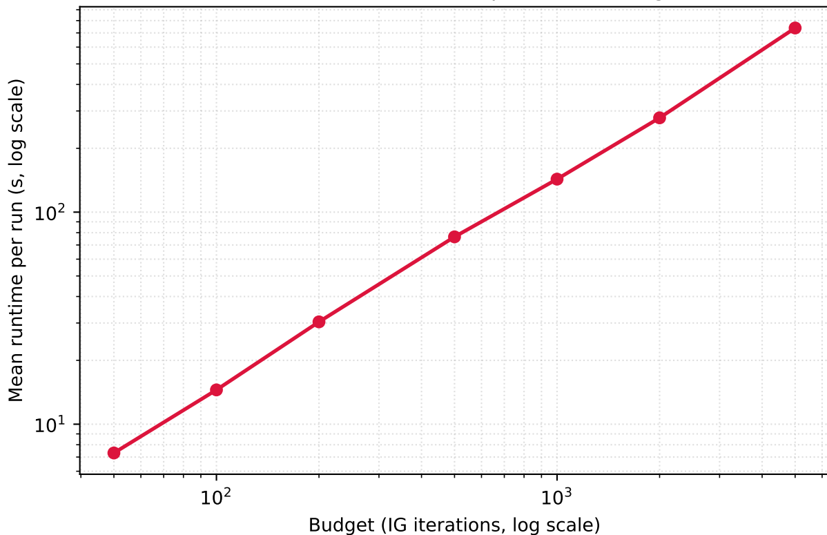
EXP-003: mean runtime per run vs budget
