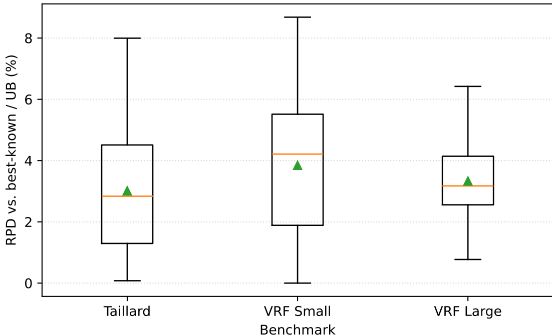
NEH baseline: RPD distribution by benchmark
