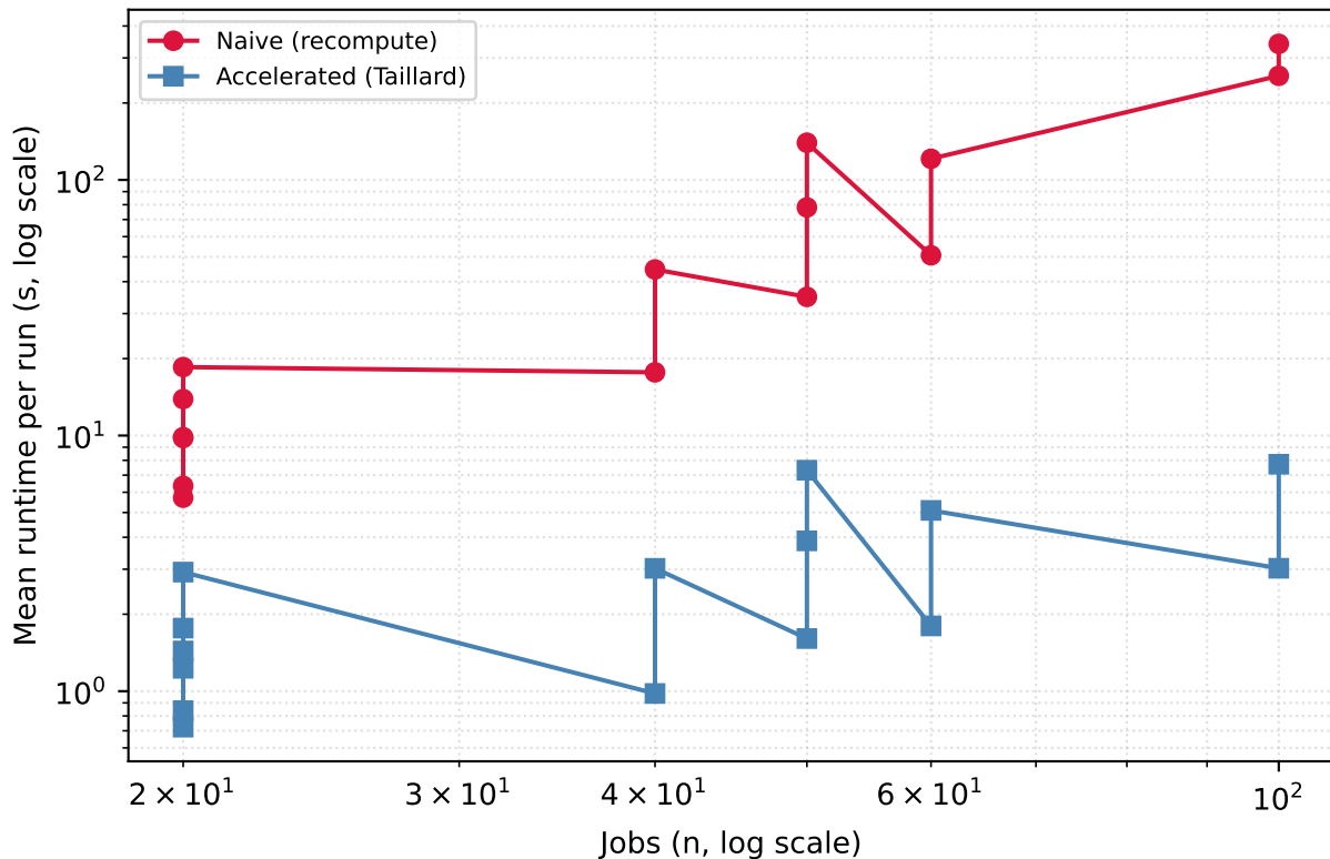
Runtime scaling: naive vs. accelerated (budget = 500)
