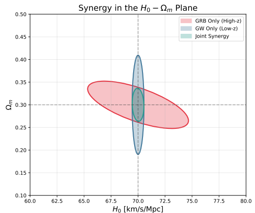
FIG. 1. Simple diagram demonstrating the concept of complementarity behind the synergies between GRB and GW observations for cosmological parameter inference.
