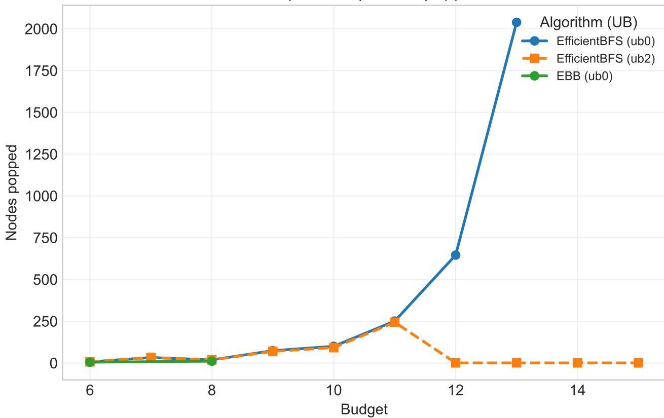
adult | \alpha=0.98 | Nodes popped
