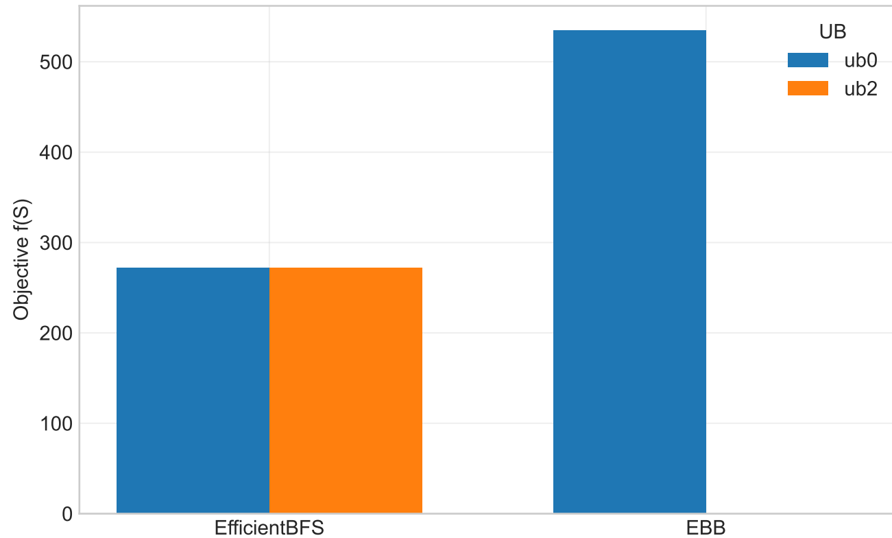
Budget 11 | Objective f(S)
