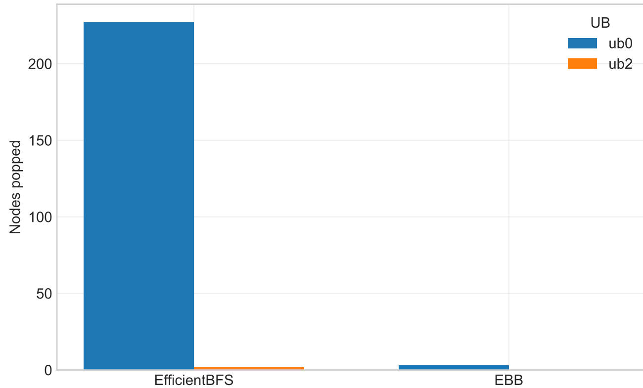
Budget 12 | Nodes popped
