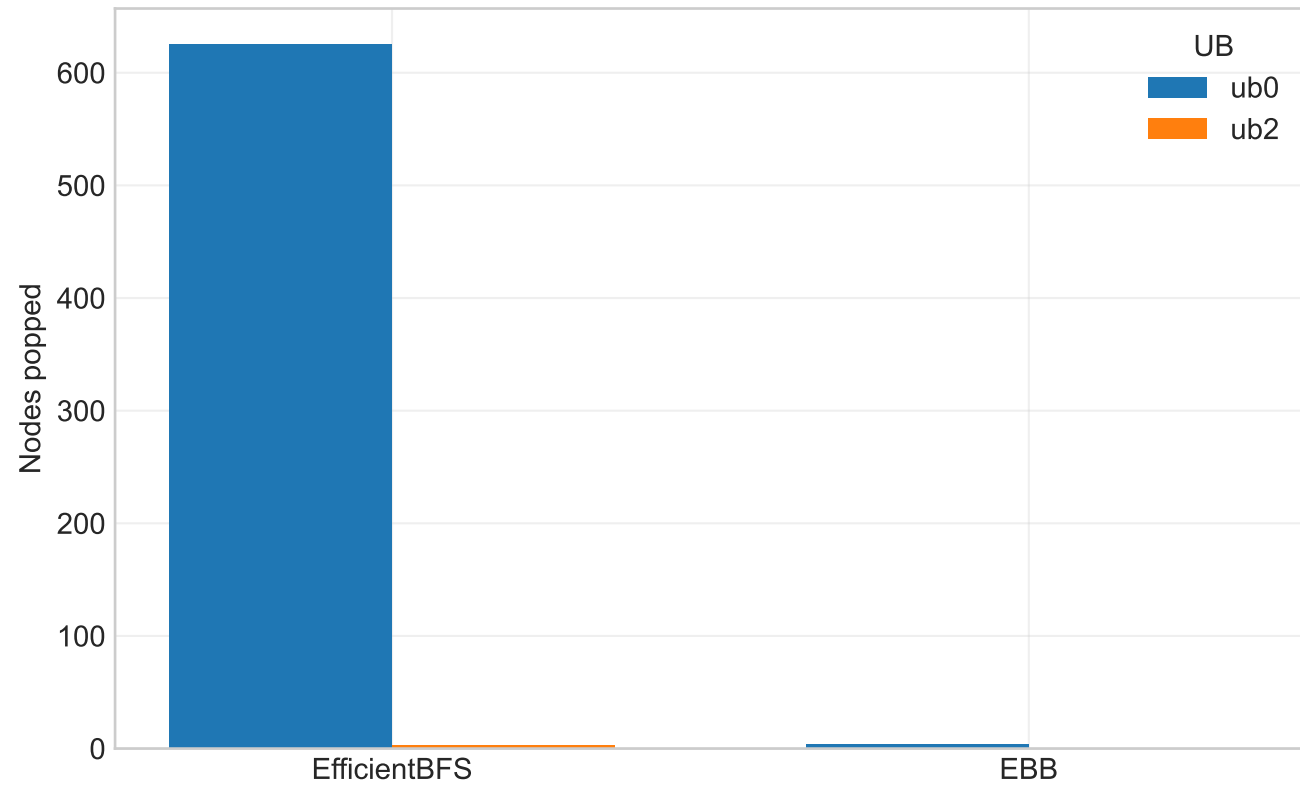
Budget 13 | Nodes popped
