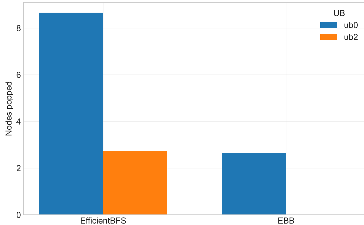
Budget 15 | Nodes popped
