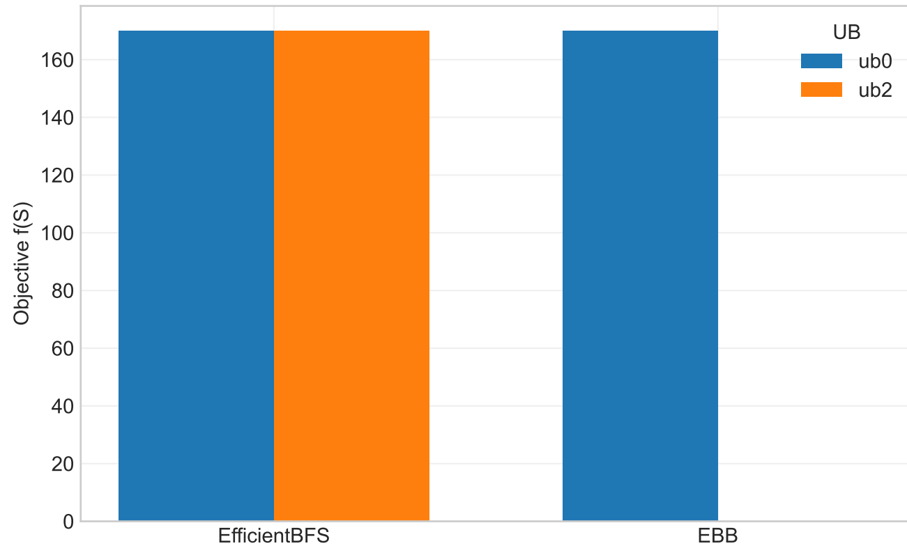
Budget 6 | Objective f(S)
