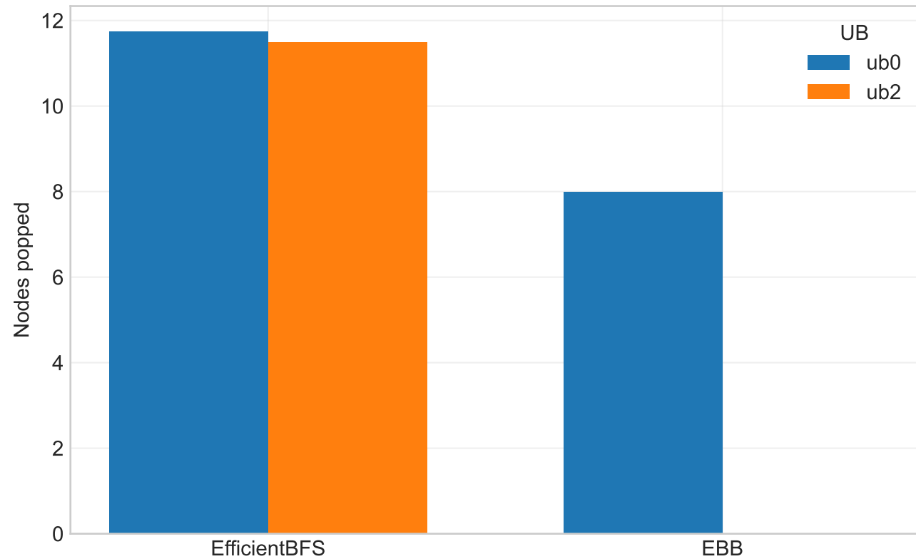
Budget 8 | Nodes popped
