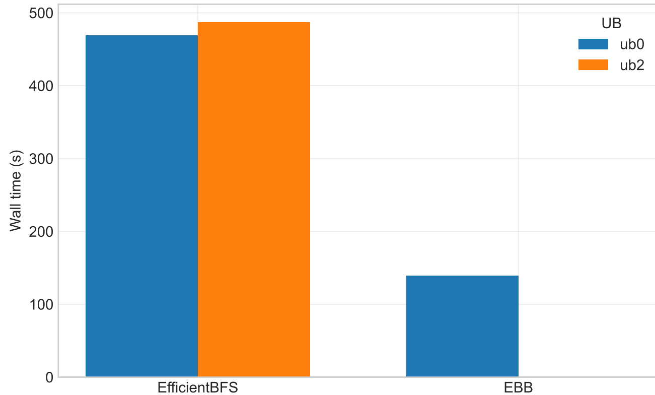
Budget 8 | Wall time (s)
