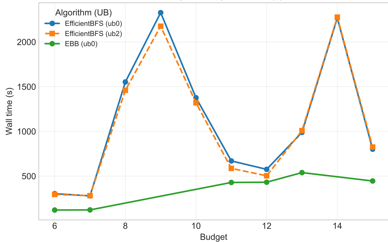
caltech | \alpha=0.98 | Wall time (s)
