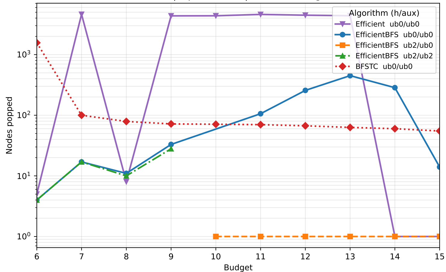
adult | \alpha = 0.95 | nodes vs budget
