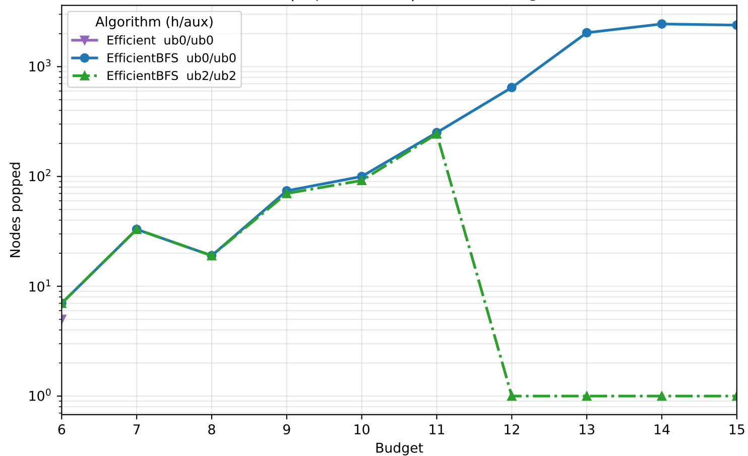
adult | \alpha = 0.98 | nodes vs budget
