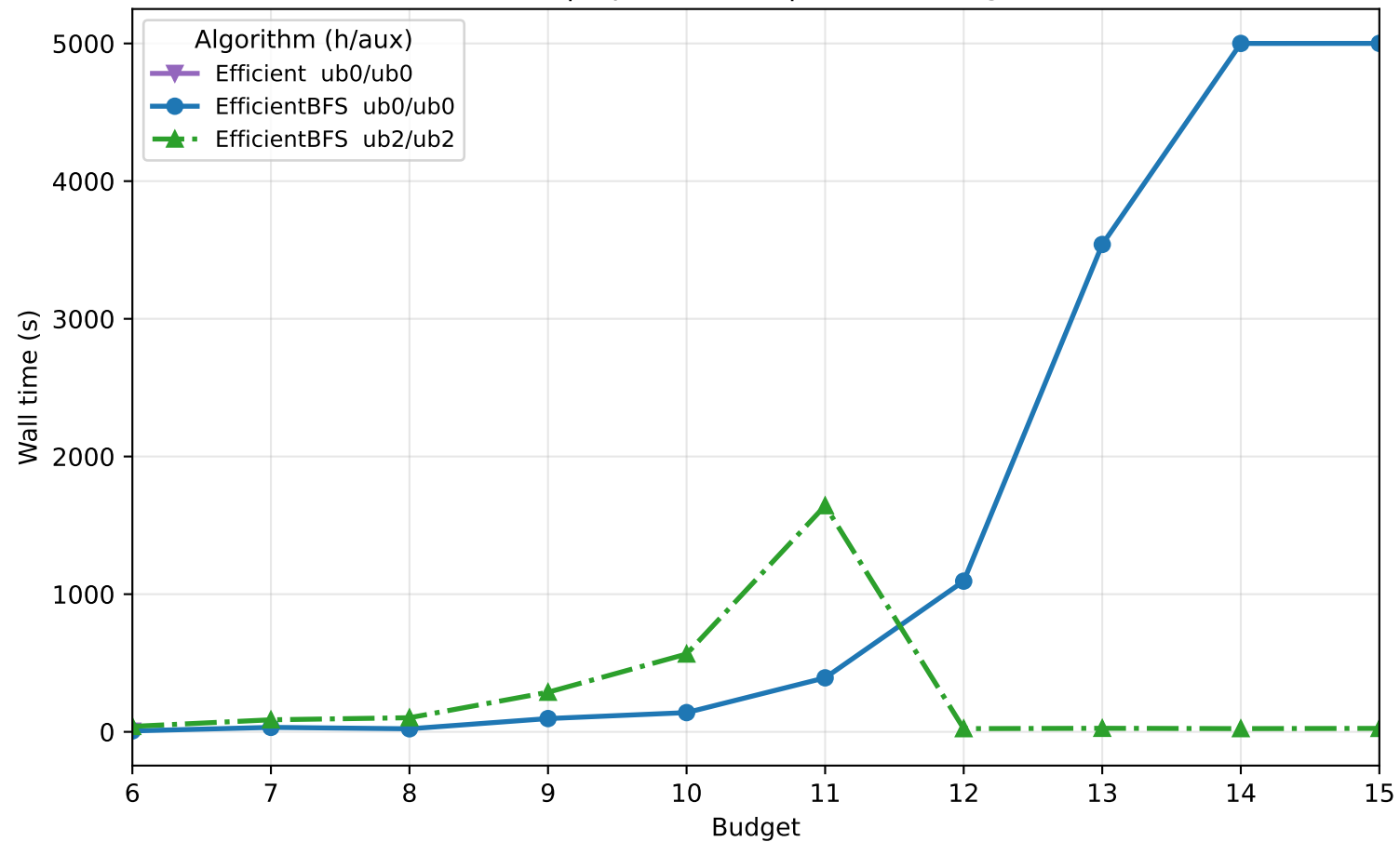
adult | \alpha = 0.98 | time vs budget
