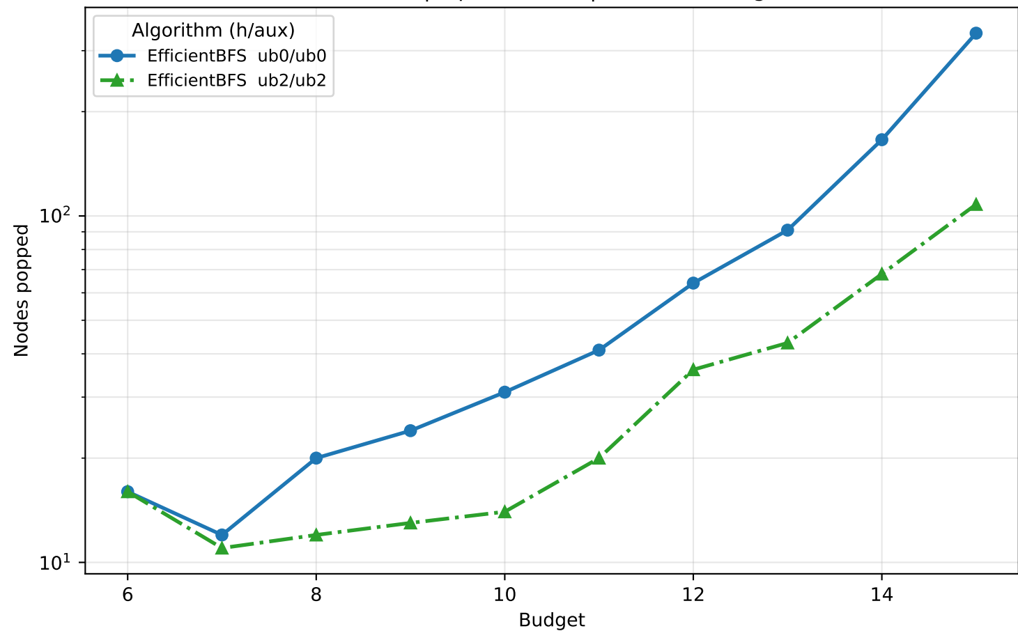
facebook | \alpha = 0.98 | nodes vs budget
