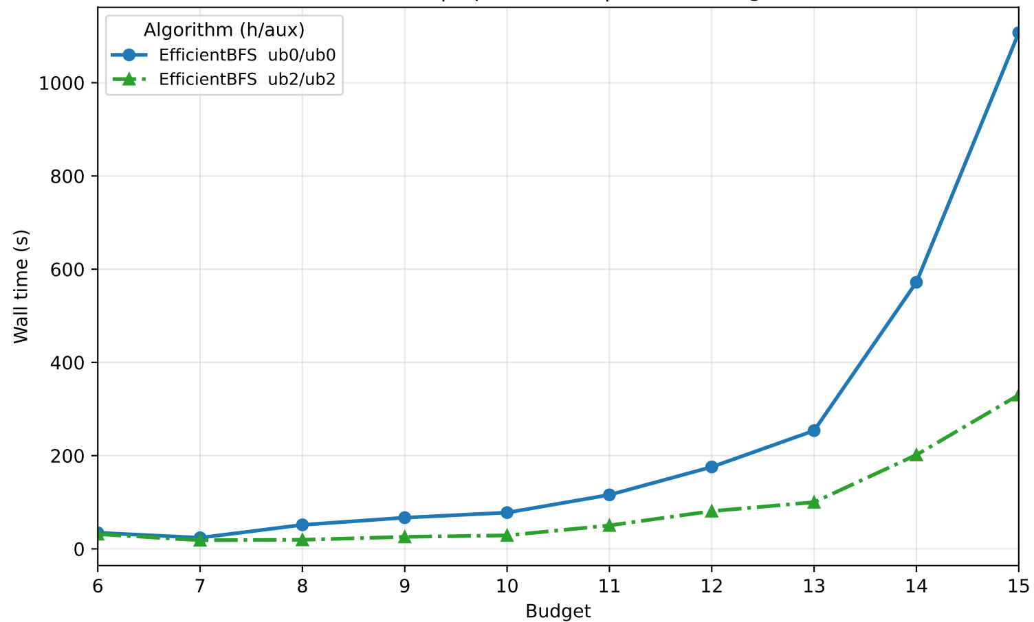
facebook | \alpha = 0.98 | time vs budget
