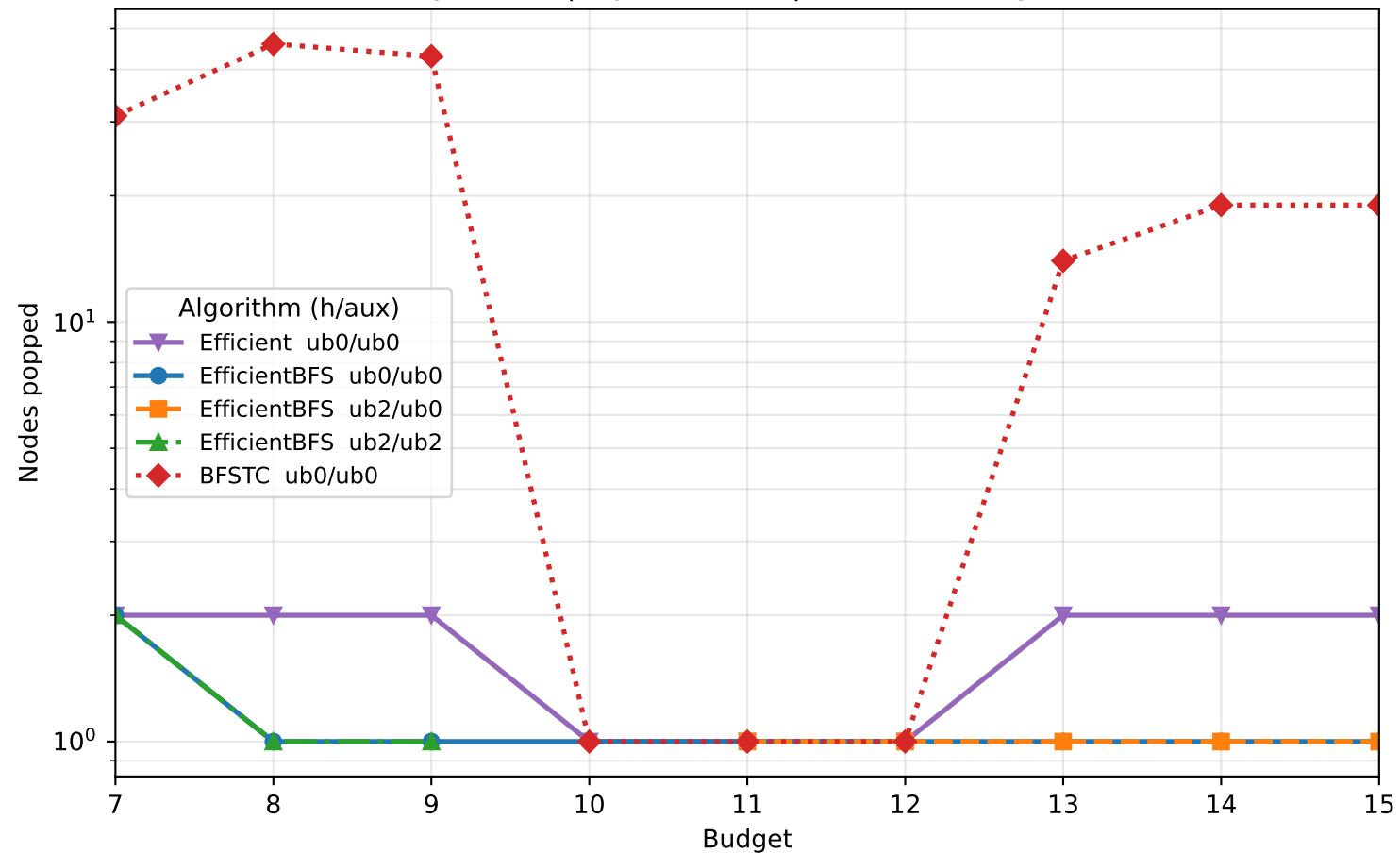
youtube | \alpha = 0.95 | nodes vs budget
