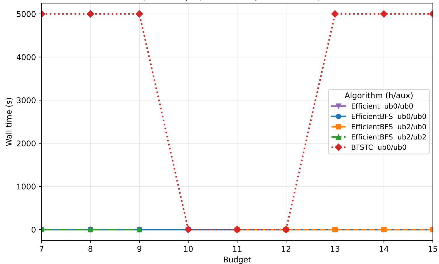
youtube | \alpha = 0.95 | time vs budget
