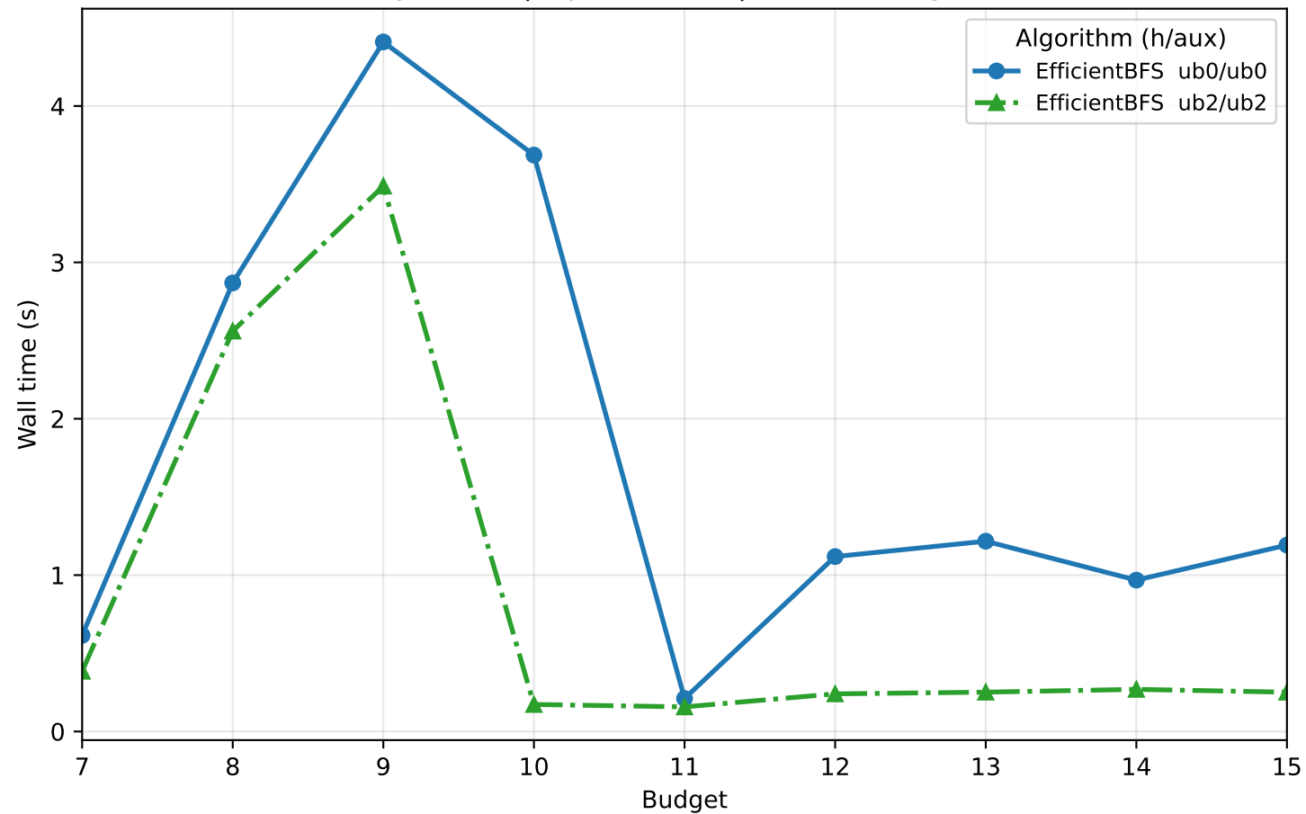
youtube | \alpha = 0.98 | time vs budget
