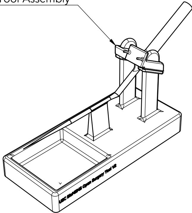
Open Surgery Tool Assembly
