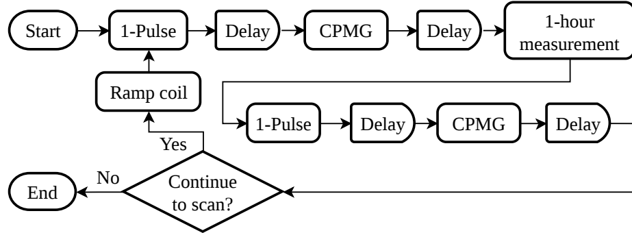
Figure 4.4: Schematic of the Earth-bound ALP measurement procedure.
