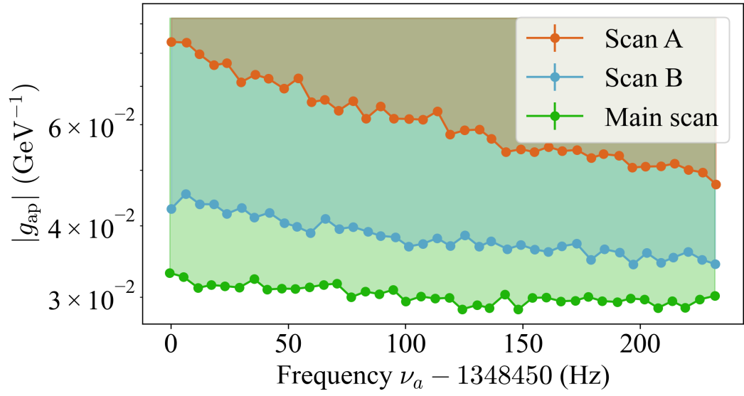
Figure 4.3: ALP gradient-proton coupling excluded at 95 % confidence level by the three sequential scans. Each data point represents the sensitivity for one scan step. The variation in sensitivity between scans reflects the daily modulation of the ALP wind direction relative to the bias field. Reproduced from Ref. [40].
