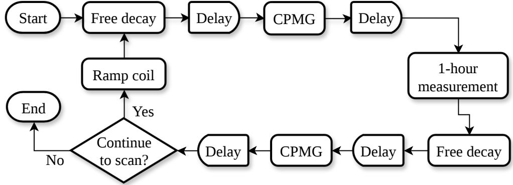
Figure 4.7: Schematic of the Earth-bound ALP measurement procedure.
