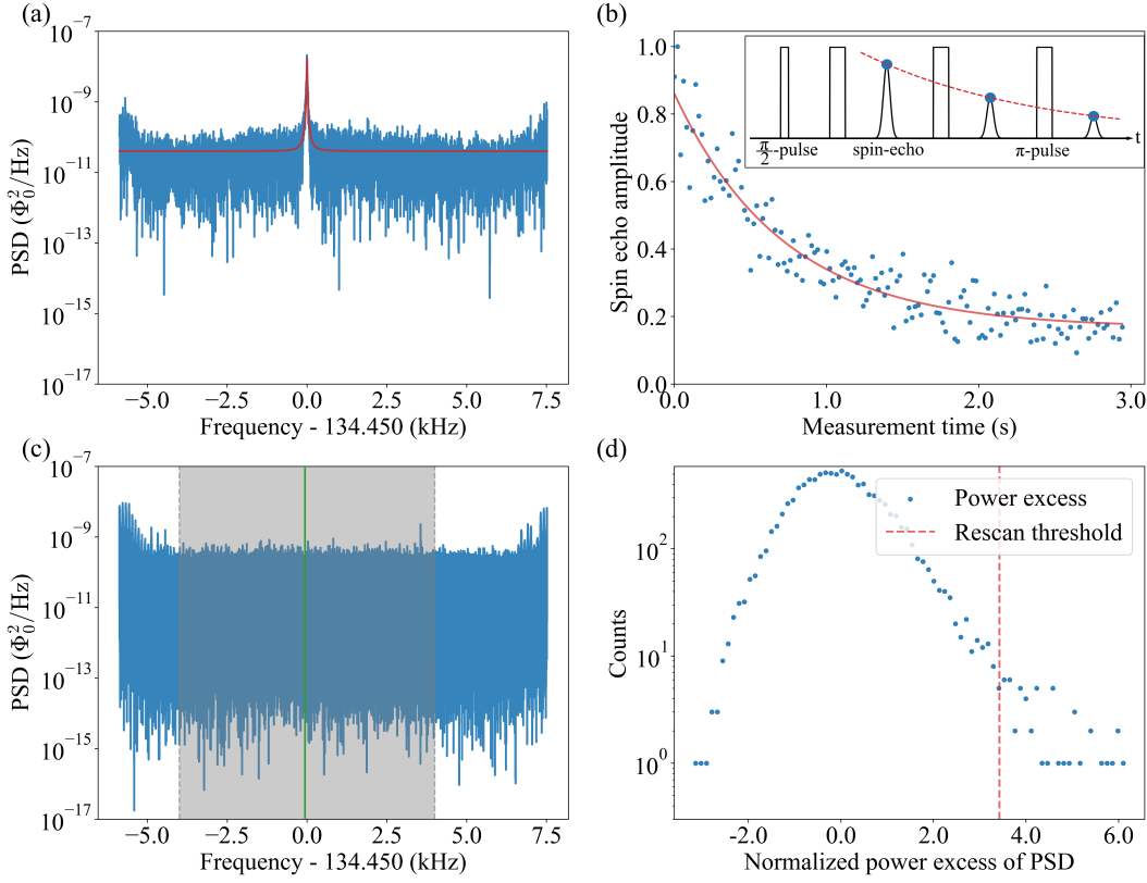
Figure 4.5: (a) PSD after a \pi/2 pulse. The NMR peak is fitted with a Lorentzian (red line); the center is at 1348 449.21(5) Hz with a FWHM of 14.79(1) Hz. (b) CPMG spin-echo amplitudes (blue dots) and exponential fit (red), giving T_2 = 0.72(5) s. (c) PSD of a 100 s ALP-search step. The gray analysis window (8 kHz wide) excludes filter artifacts near the band edges; the green resonant window ( \pm 5 NMR linewidths = \pm 70 Hz) is where ALP signal candidates are sought. (d) Histogram of normalized power excess (NPE) derived from (c), with the rescan threshold \Theta_{\text{RE}} (red line) at the 95 % confidence level for a 5\sigma ALP detection. Reproduced from Ref. [38].
