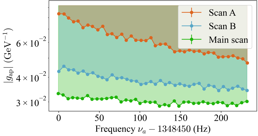
Figure 4.6: ALP gradient-proton coupling excluded at 95 % confidence level by the three sequential scans. Each data point represents the sensitivity for one scan step. The variation in sensitivity between scans reflects the daily modulation of the ALP wind direction relative to the bias field. Reproduced from Ref. [38].
