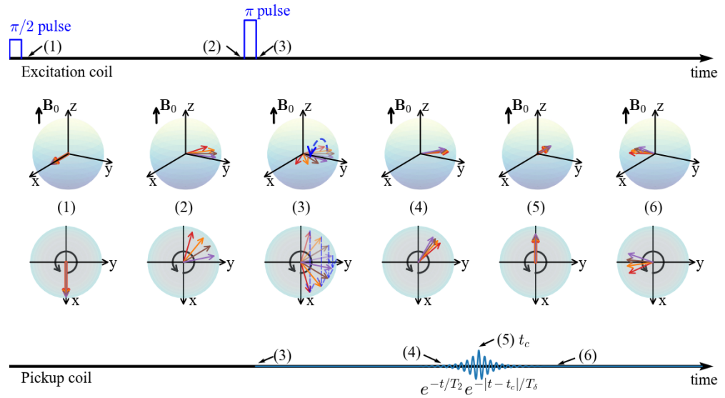
Figure 1.3: Schematic of the spin-echo sequence in the laboratory frame. The \pi pulse reverses dephasing from static field inhomogeneity, producing an echo at time 2\tau .
