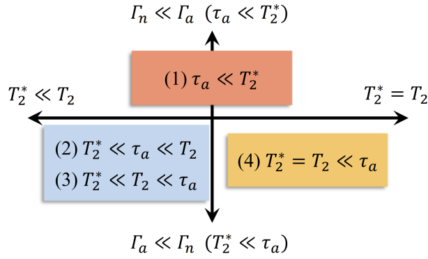
Figure 2.1: Regimes of the spin-precession experiment based on the relative magnitudes of T_2 , T_2^* , and \tau_a . Reproduced from Ref. [44].
