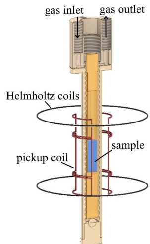
Figure 3.2: The methanol sample (blue) sits at the center of the three-coil Nb saddle-pair pickup (red). Helmholtz coils (black) fine-tune the bias magnetic field. Adapted from Ref. [64] with permission.
