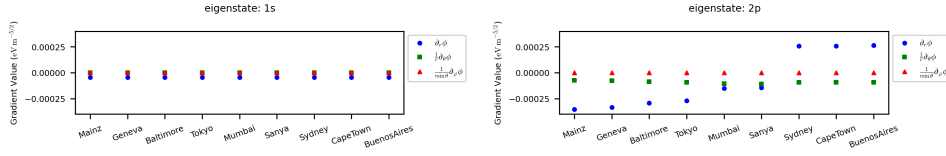
Figure 2.5: gradients of 1s 2p... states. Three rows would be enough. Yuzhe: mention the time for computing the gradients.
