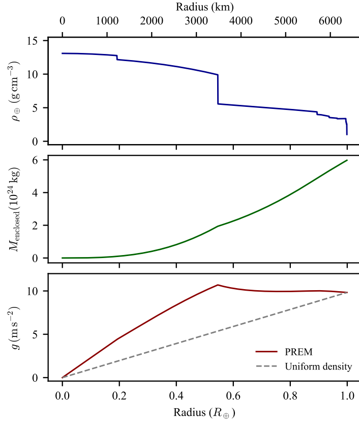
Figure 2.4: Earth’s density (top), enclosed mass (middle), and gravitational acceleration magnitude (bottom) as functions of radius according to PREM [0]. The acceleration is calculated as g(r) = GM_{\text{enclosed}}(r)/r^2 , with g(0) = 0 . The dashed curve shows the linear interior profile of a uniform-density sphere with the same total mass and radius.
