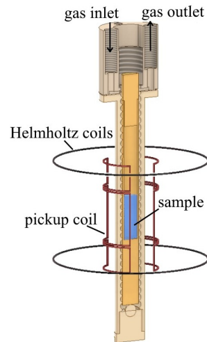
Figure 3.2: The methanol sample (blue) sits at the center of the three-coil Nb saddle-pair pickup (red). Helmholtz coils (black) fine-tune the bias magnetic field. Adapted from Ref. [0] with permission.
