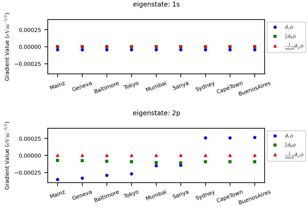
Figure 2.5: gradients of 1s 2p... states. Three rows would be enogh.
