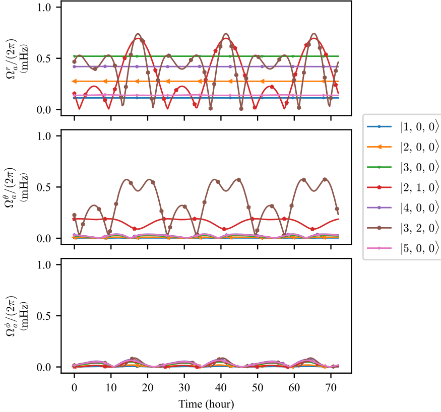
Figure 4.10: Expected daily modulation of the ALP signal for the seven lowest-energy eigenstates ( m = 0 ) of the Earth-bound ALP halo, where the ALP density is significant at Earth radius. ALP Compton frequency is taken as 1.348 500 MHz. Lorentz boost is considered. The quantization axis is arbitrarily chosen to be along the Earth–Sun line.
