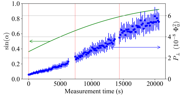
Figure 4.5: ALP parameters modulated by Earth’s motion. Plotted for the start times of each measurement step for each of the three scans in seconds. Zero time corresponds to start of the data taking on December 23, 2022, 15:47:30 (Central European Time, UTC+1). Vertical dashed red lines mark the beginning time of a scan. Green line: \sin \alpha oscillates with a period of one day. Blue dot with error bar: expected ALP signal powers in the PSD, according to Equations (3.2) and (3.3), for the reference case of an ALP gradient coupling to proton of g_{\text{ap}} = 10^{-9} \text{ GeV}^{-1} . Uncertainties for these values were propagated from errors of the spin relaxation times T_2 and T_2^* , sample Larmor frequency and NMR signal power. Reproduced from Ref. [59] with permission.
