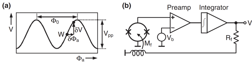
Figure 3.4: (a) V - \Phi characteristic of dc-SQUID showing the operating point W where the feedback voltage has approximately linear dependence on magnetic flux. (b) Direct-coupled FLL circuit with built-in pre-amplifier and integrator for maintaining the SQUID at the linear operating point. Reproduced from [squidhandbookintro] with permission.
