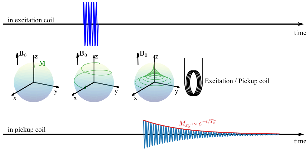
Figure 1.2: Schematic of free-decay pulsed NMR sequence in the laboratory frame. One excitation pulse tips the magnetization into the transverse plane, where it precesses and decays with time constant T_2^* . The signal is measured by a pickup coil.
