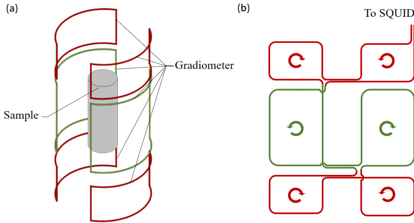
Figure 3.3: (a) Simplified schematic of gradiometer and sample positioned at the center. (b) Details of gradiometer loop connection showing the three-coil saddle-pair configuration with opposing windings for noise rejection.
