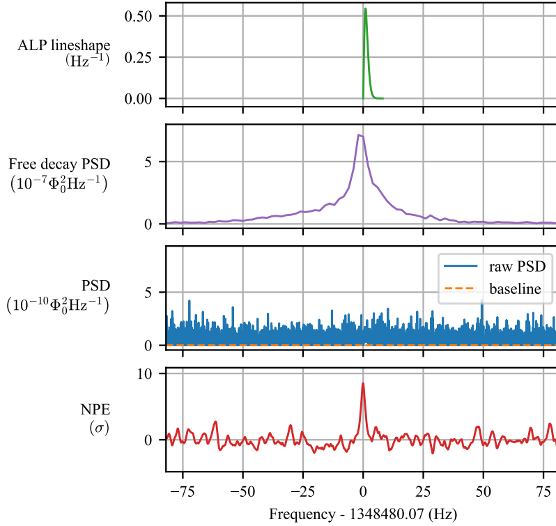
Figure 4.6: Example of data processing with fake ALP signal injected at the center of the spectrum. Top to bottom: lineshape of normalized ALP field, free decay PSD, PSD of the measurement, and NPE.
