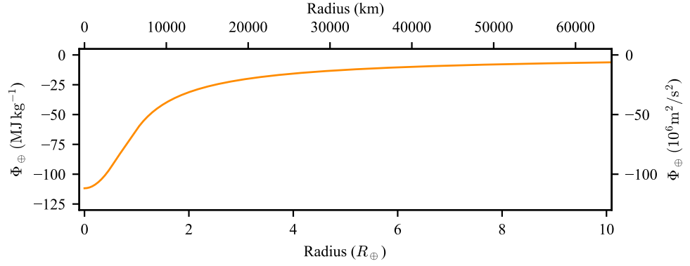
Figure 2.5: Earth gravitational potential over radius considering the density profile.
