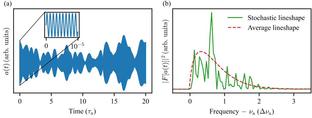
Figure 2.1: Simulated axion fields in the time and frequency domains. (a) Time-domain axion field a(t) , with a magnified view showing the oscillation at axion Compton frequency in the inset. The envelope of the a(t) changes over time, indicating the coherence time \tau_a is finite. Here \tau_a is chosen as Q_a/\nu_a . (b) The stochastic lineshape in the frequency domain is computed as |F[a(t)]|^2 , where F[a(t)] denotes the Fourier transform of the time-domain signal shown in (a). The average lineshape represents the expected amplitude spectrum after sufficient averaging. The linewidth \Delta\nu_a is approximated as \nu_a/Q_a . Reproduced from Ref. [7], originally prepared by the author.
