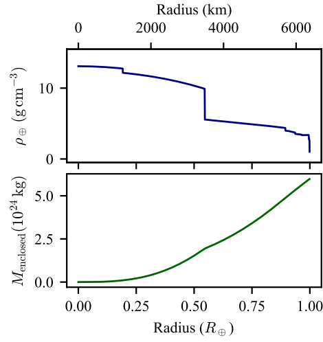
Figure 2.4: Earth density (upper plot) and enclosed mass (lower plot) over radius according to PREM [25].
