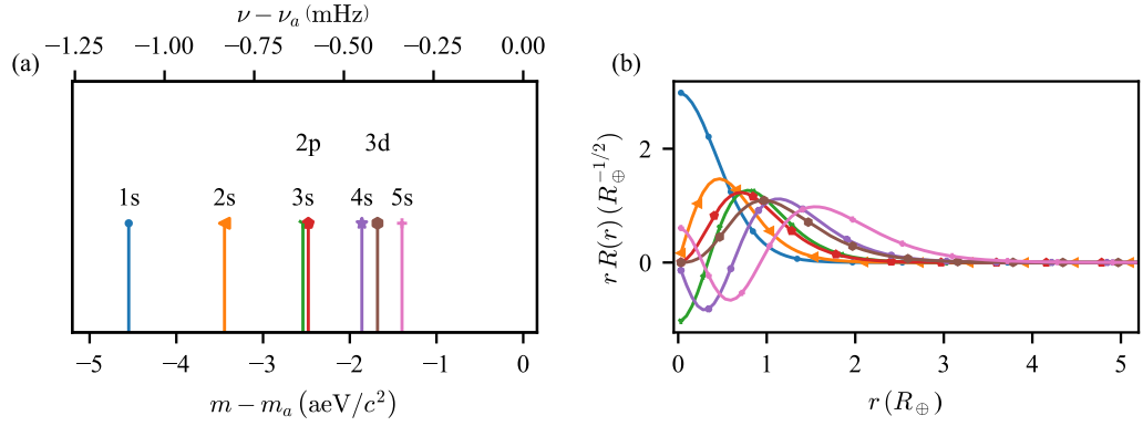
Figure 2.6: The lowest seven eigen-states derived from TISE assuming 1 MHz axion Compton frequency. (a) Eigen-energies converted to masses and frequencies compared to the axion rest mass and Compton frequency. (b) The corresponding reduced radial wavefunctions (radius times the radial wavefunction) using the same color and marker scheme as in (a).
