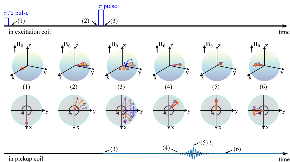
Figure 1.3: Schematic of the spin-echo sequence in the laboratory frame. Black circular arrows indicate the precession. Colorful arrows stand for magnetization of small sample packets precessing at different Larmor frequencies. The \pi pulse reverses dephasing from static field inhomogeneity and produce echos. The indices in brackets indicate the time sequence of the pulses and echos.
