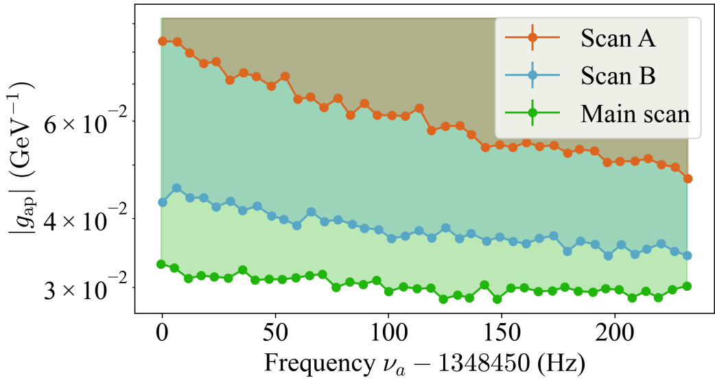
Figure 4.8: ALP gradient-proton coupling excluded at 95 % confidence level by the three sequential scans. Each data point represents the sensitivity for one scan step. The variation in sensitivity between scans reflects the daily modulation of the ALP wind direction relative to the bias field. Reproduced from Ref. [38].
