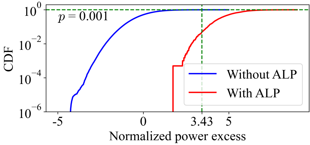
Figure 4.7: Empirical cumulative distribution function of the filtered NPE. The vertical dashed line marks the rescan threshold \Theta_{\text{RE}} , chosen to recover a 5\sigma ALP signal with 95 % probability. The corresponding noise-only tail probability (horizontal dashed line) is approximately 0.001.
