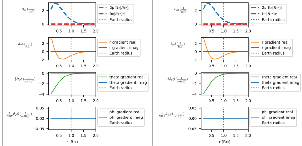
Figure 2.5: gradients of 1s 2p... states. Three rows would be enough.
