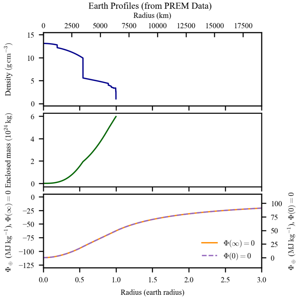
Figure 2.4: Earth density, mass, and gravitational potential profiles from PREM [25].
