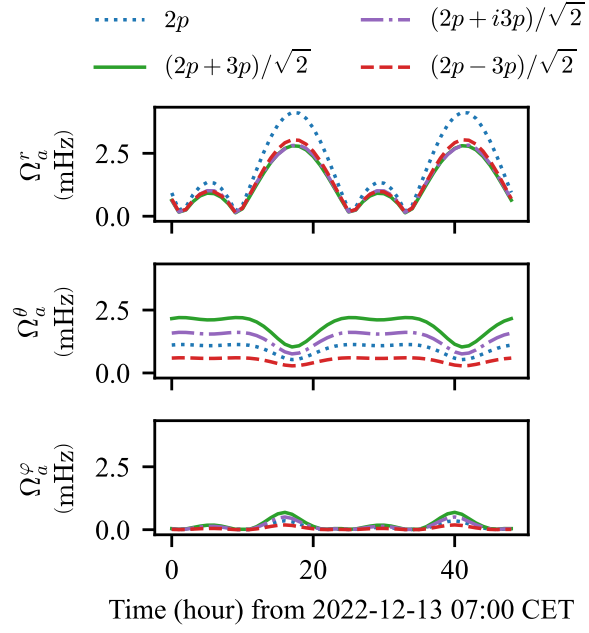
Figure 4.11: Expected evolution of the ALP-induced Rabi frequencies for the Earth-bound ALP halo model. Top to bottom: Rabi frequencies induced by gradients and Lorentz boost in radial, polar, and azimuthal directions. Scenarios of different state populations are considered as shown in the legend. The amplitude modulation is driven by the rotation of the laboratory frame relative to the ALP-field gradient. Yuzhe: highlight the course of the measurement in the figure.
