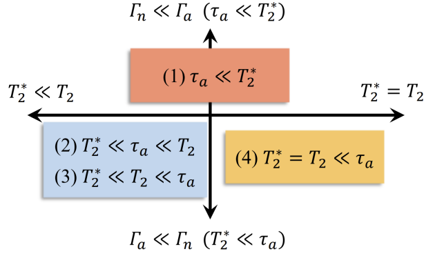
Figure 2.1: Regimes of the spin-precession experiment based on the relative magnitudes of T_2 , T_2^* , and \tau_a . Reproduced from Ref. [37].
