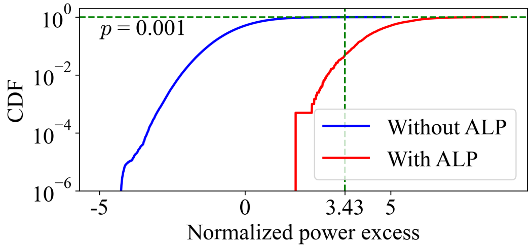
Figure 4.8: Empirical CDF obtained from the NPE distribution of spectra. The vertical dashed line represents the threshold for rescanning, \Theta_{RE} , corresponding to the null hypothesis of a 5\sigma ALP detection at the 95% confidence level. The p-value corresponding to the threshold (horizontal dashed line) is approximately 0.001.
