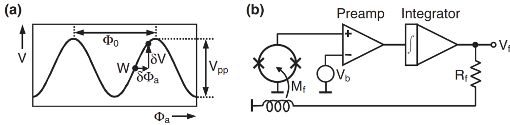
Figure 3.4: (a) V - \Phi characteristic of dc-SQUID showing the operating point W where the feedback voltage has approximately linear dependence on magnetic flux. (b) Direct-coupled FLL circuit with built-in pre-amplifier and integrator for maintaining the SQUID at the linear operating point.
