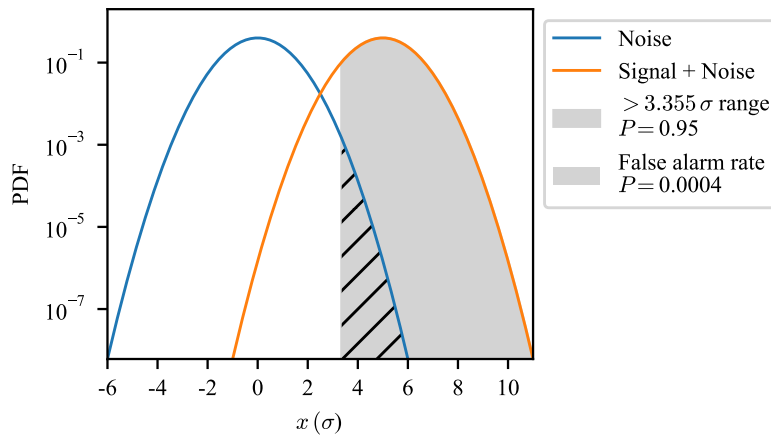
Figure 4.3: Noise and signal amplitude distributions assuming Gaussian noise and linear signal dependence.
