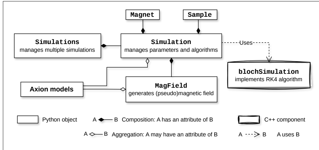
Figure A.1: Architecture of axionbloch. Each Simulation instance receives parameters from Magnet , Sample , and MagField . For axion simulations, an axion-model object is required both to configure the simulation and to generate the pseudomagnetic field. Numerical integration is performed via the blochSimulation API, which provides Python access to the C++ backend. Reproduced from Ref. [64], originally prepared by the author.
