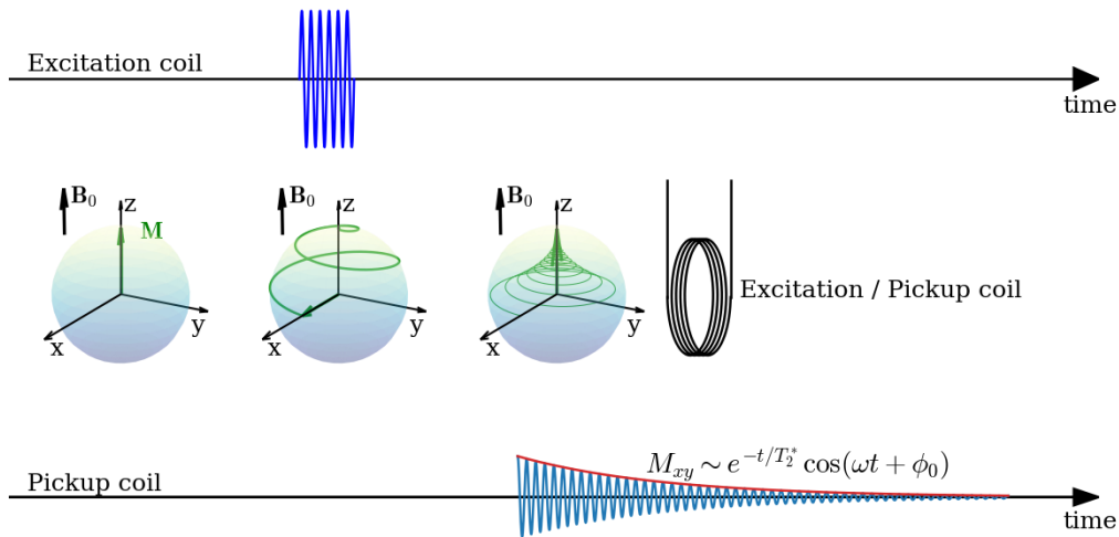
Figure 1.2: Schematic of pulsed NMR sequences in the laboratory frame.
