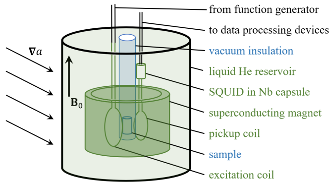
Figure 1.4: Conceptual diagram of the CASPER-Gradient-Low-Field setup. Superconducting devices (dark green) are submerged in a liquid helium bath (light green). The excitation and pickup coils characterize the sample and detect the spin-precession signal. The sample temperature can be controlled independently of the helium bath, enabling measurements with both thermal and hyperpolarized samples. Reproduced from Ref. [49].
