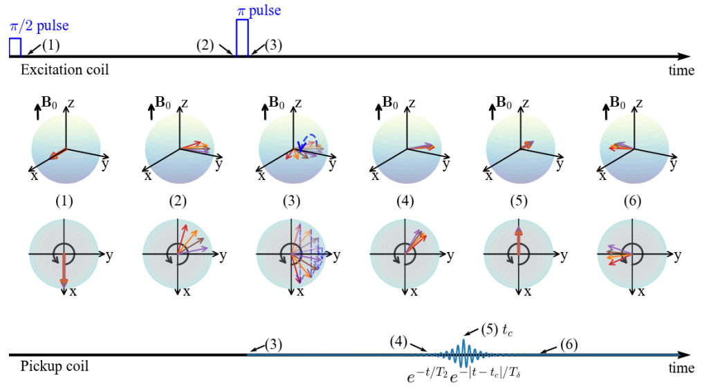
Figure 1.3: Schematic of the spin-echo sequence in the laboratory frame. The \pi pulse reverses dephasing from static field inhomogeneity, producing an echo at time 2\tau . Yuzhe: modify the pic
