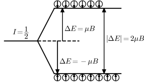
Figure 1.1: Zeeman splitting of a spin-1/2 nucleus in a magnetic field B . The energy difference \Delta E between the two spin states is proportional to B . Yuzhe: TODO edit equation in the figure.
