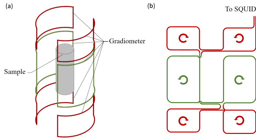
Figure 3.2: (a) Simplified schematic of gradiometer and sample positioned at the center. (b) Details of gradiometer loop connection showing the three-coil saddle-pair configuration with opposing windings for noise rejection.
