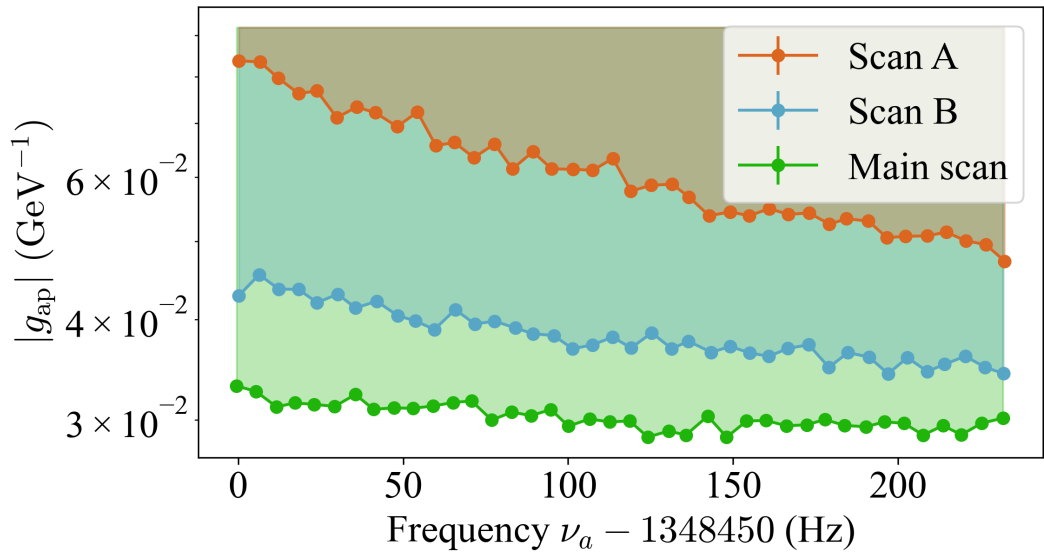
Figure 4.9: ALP gradient-proton coupling excluded at 95 % confidence level by the three sequential scans. Each data point represents the sensitivity for one scan step. The variation in sensitivity between scans reflects the daily modulation of the ALP wind direction relative to the bias field. Reproduced from Ref. [38].
