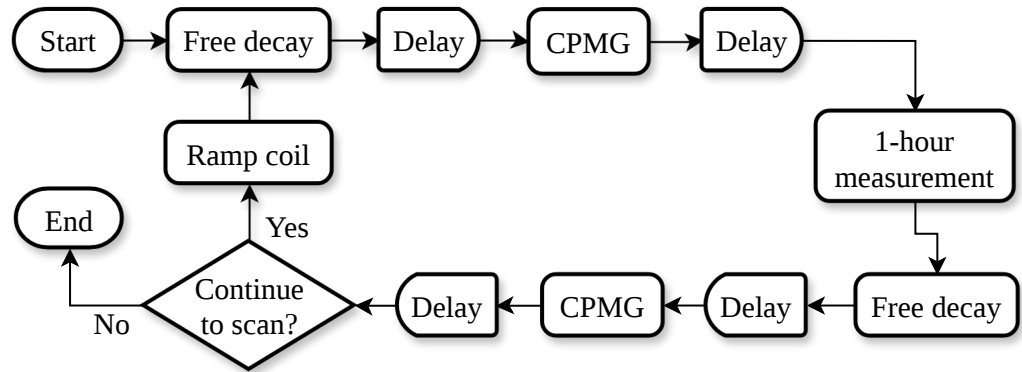
Figure 4.10: Schematic of the Earth-bound ALP measurement procedure.
