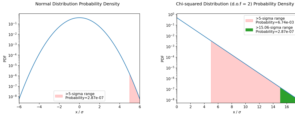
Figure 4.2: (a) The probability of a Gaussian random variable exceeding n times of its standard deviation. The probability of a 5 - \sigma signal is less than 2.87 \times 10^{-7} . (b) The \chi^2 distribution with two degrees of freedom. Yuzhe: to be updated
