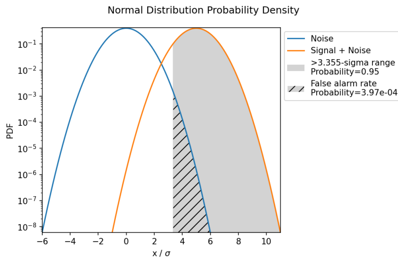
Figure 4.3: Noise and signal amplitude distributions assuming Gaussian noise and linear signal dependence. Yuzhe: to be updated
